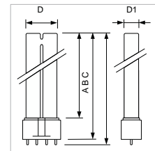
Osram PL-L 18W/71/4P
