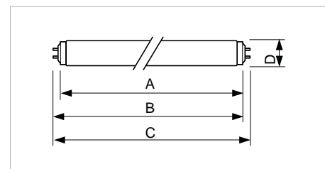
Dimensions with bi-pin cap (G13)
